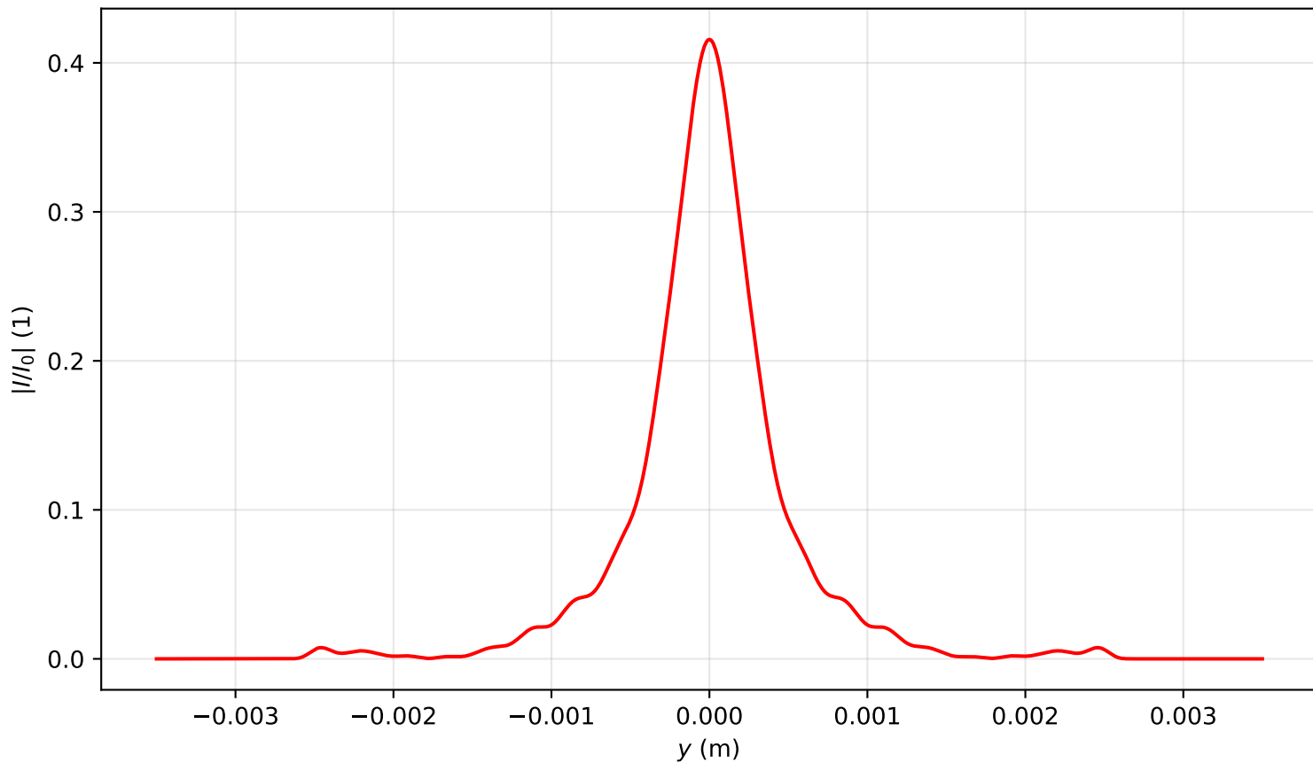
Intensity profile I(x=0, y, z=1.751)/I_0 , P_{in}=3.0P_{cr} , artificial time
